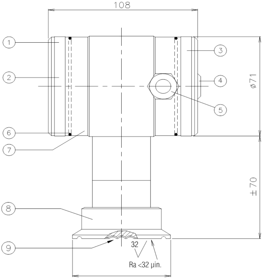
1,5" or 2" TRI CLAMP
